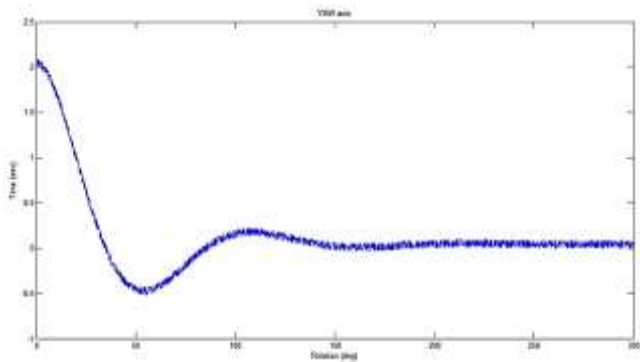
Fig. 14. X-axis position stabilization with LQR controller with integrator and perturbation.
