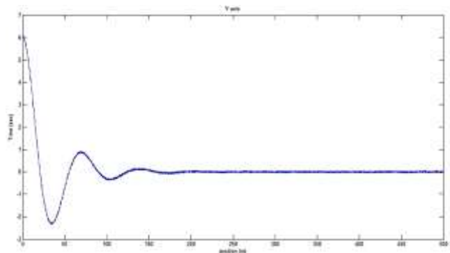
Fig. 7. Y-axis position stabilization with LQR controller without perturbation.
